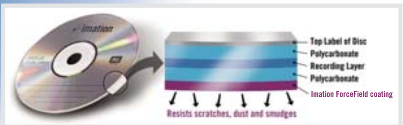
Cross section of Imation DVD protected by ForceField coating
